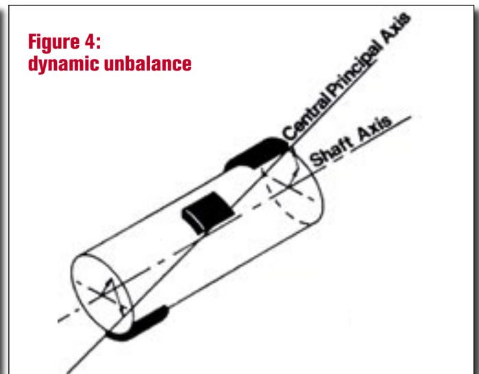
Figure 4: dynamic unbalance No intersect at all between the principal axis and the rotating centreline
