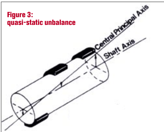
Figure 3: quasi-static unbalance A similar offset to couple unbalance but with the intersect not at the c of g
